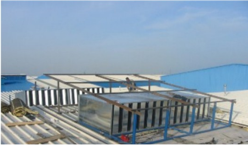
Trakya Cam San.A.Ş. Automotive Glass department Lüleburgaz Plant Fan room sound insulation application
